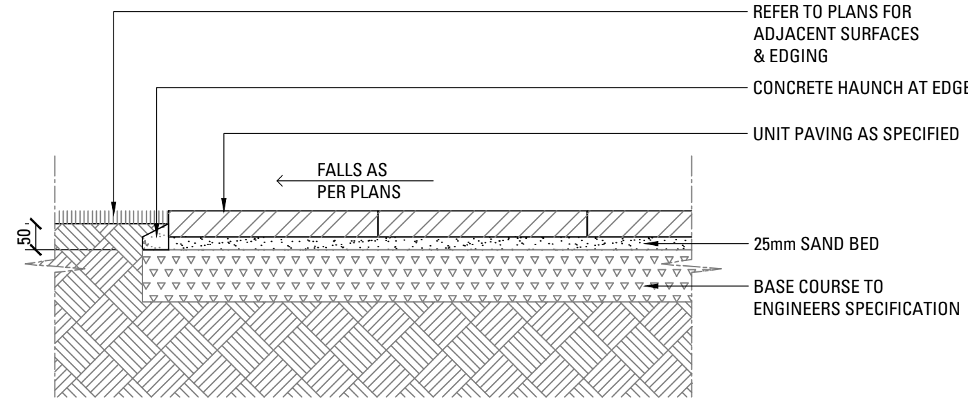
02 UNIT PAVERS ON GRADE SCALE 1:10
