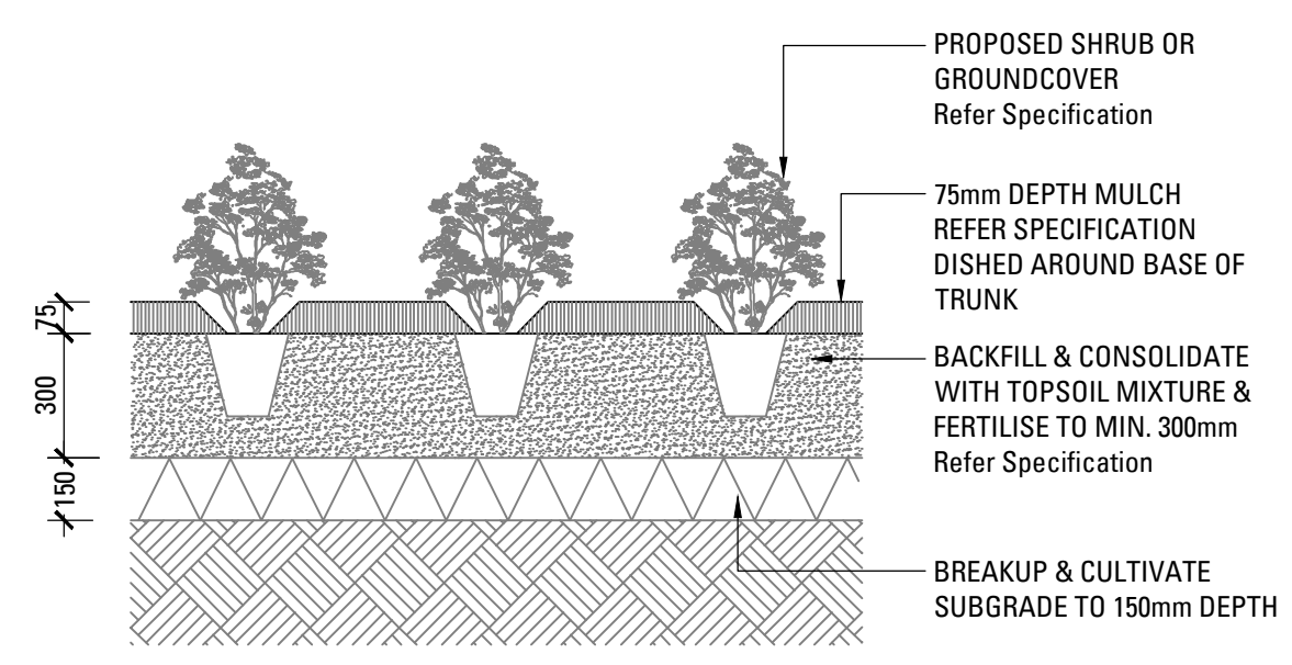
05 SHRUB OR GROUND COVER IN PLANTING BED SCALE 1:20
