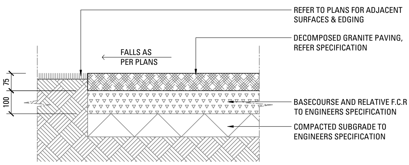
03 DECOMPOSED GRANITE PAVING ON GRADE SCALE 1:10
