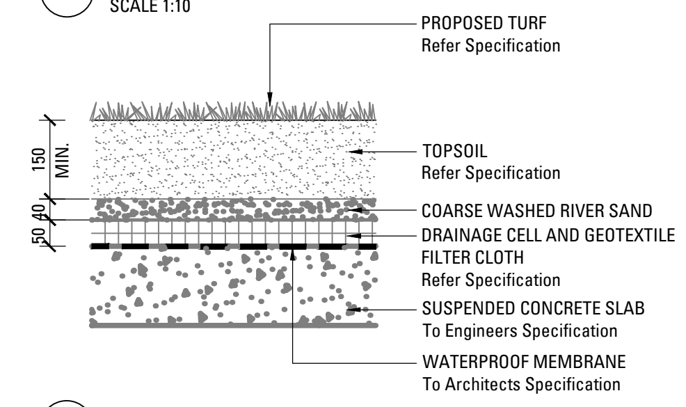
07 TURF ON SLAB SCALE 1:10
