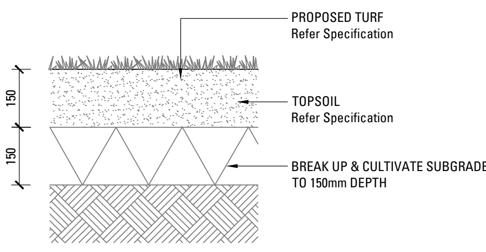
06 TURF ON GRADE SCALE 1:10
