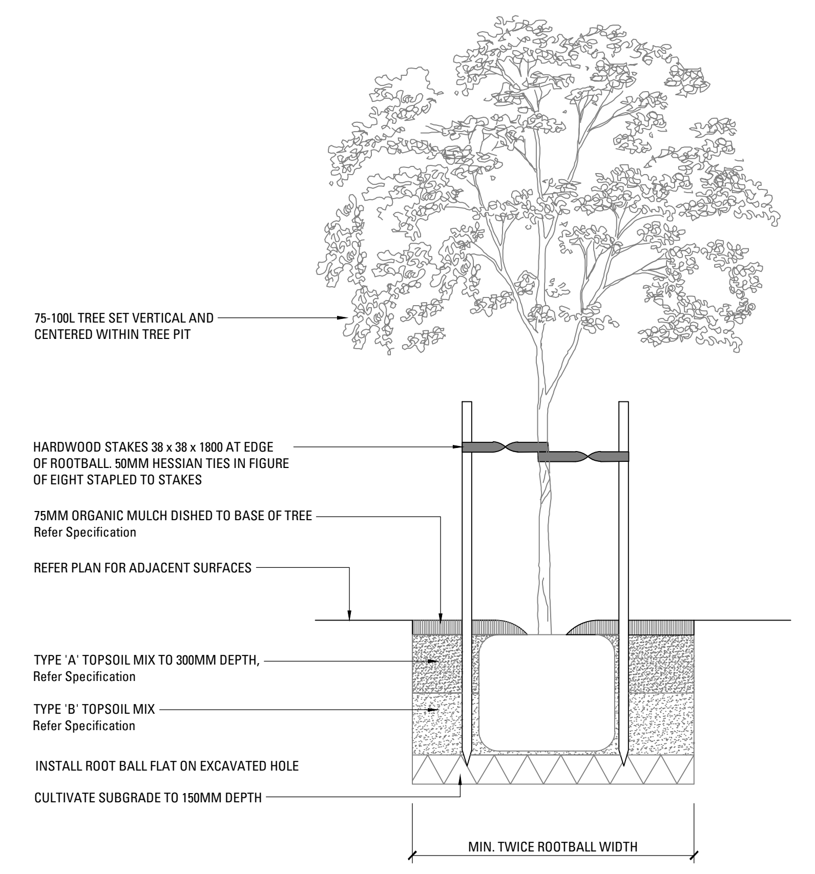
04 TREE PLANTING 75-100L SCALE 1:20
