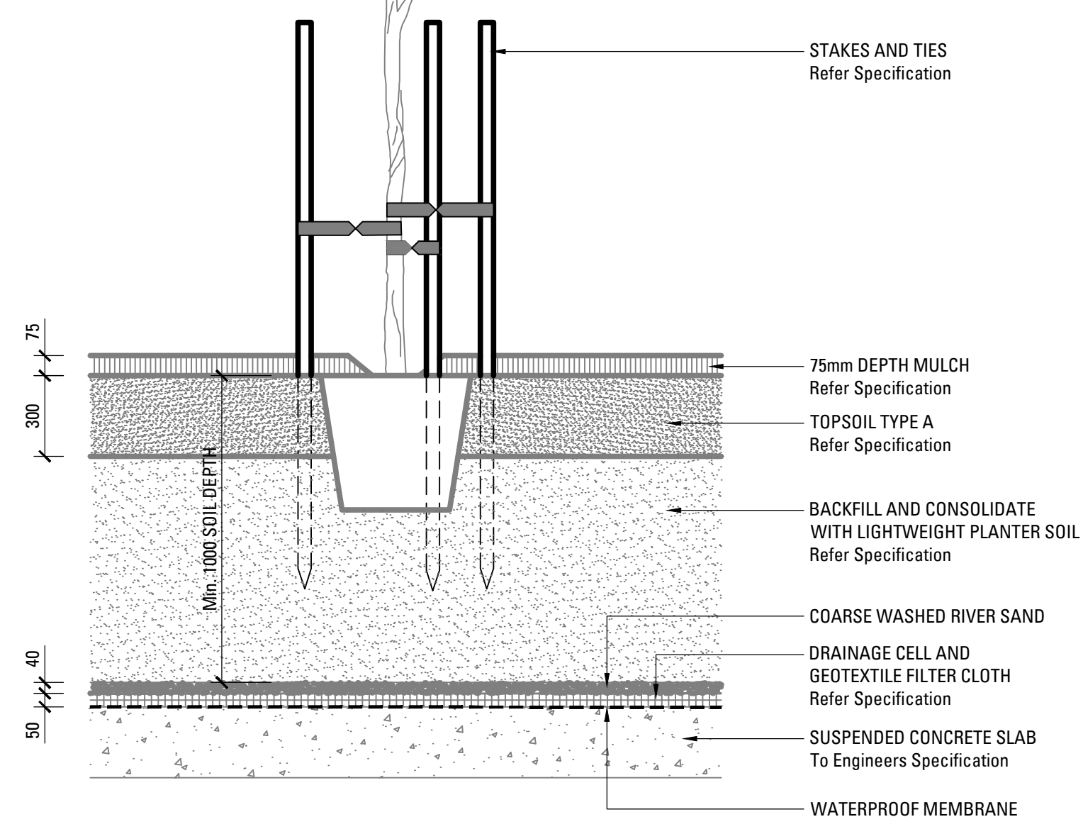
08 TREE PLANTING ON SLAB 75-100L SCALE 1:20
